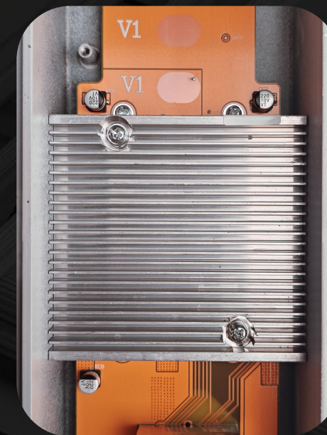
Receiver Card Heat Dissipation (Optional)
